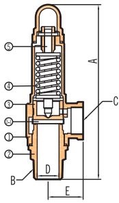
N9B Type Sealing ½"~2"
