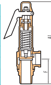
N9LB Type Lever ½"~2"
