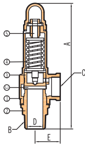
N9B Type Sealing ½"~2"
